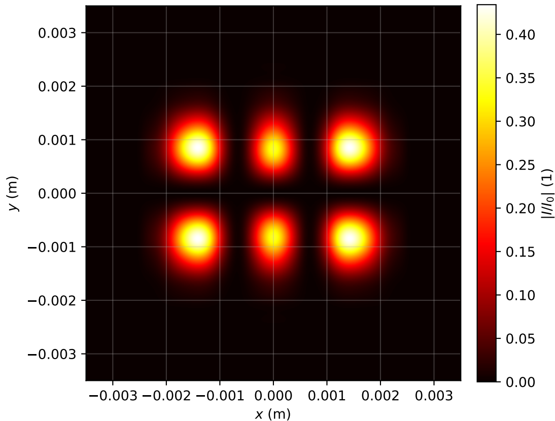
Intensity profile I(x, y, z = 3.025)/I_0 , P_{in}=2.0P_{cr} , artificial time
